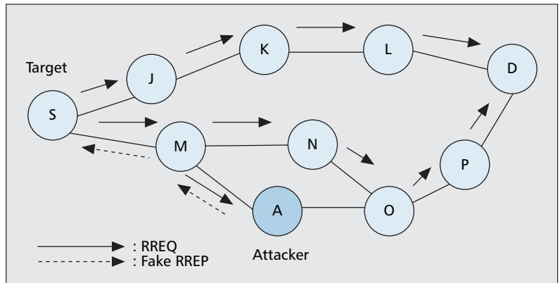
■ Figure 1. Example of a blackhole attack on AODV.
