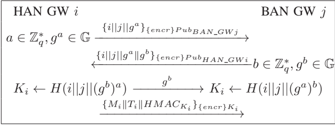
Fig. 4. Proposed lightweight message authentication scheme
