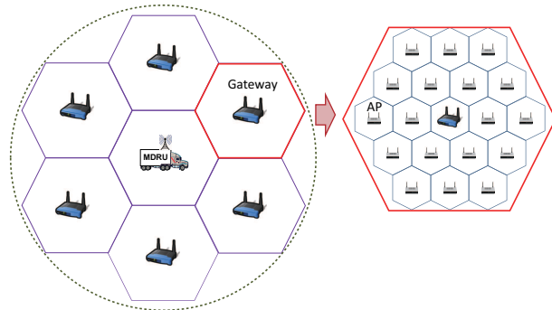
(a) Considered scenario with 7 hexagonal cells in the coverage of one MDRU.
